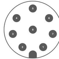
LaserLink Connector: M8 8-Pin A-Coded Female
